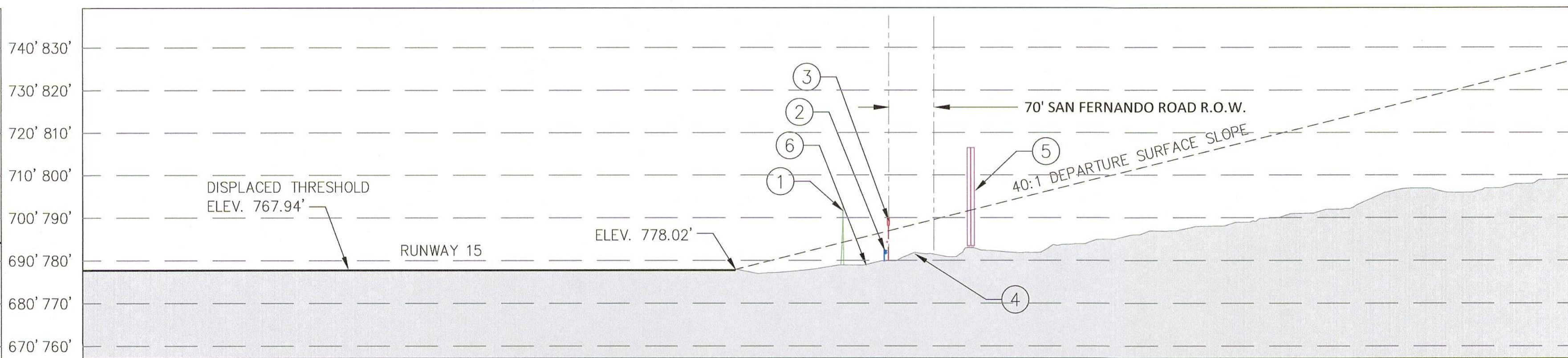
RUNWAY 15 END DEPARTURE PROFILE VIEW (On Centerline)
