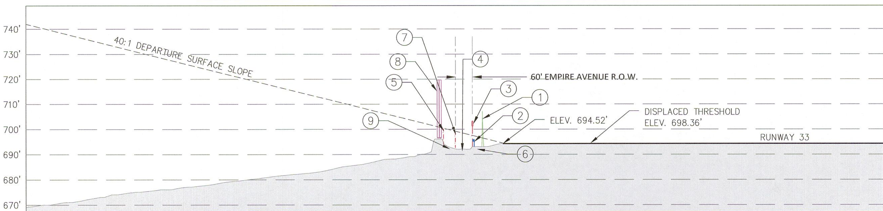
RUNWAY 33 END DEPARTURE PROFILE VIEW (On Centerline)
